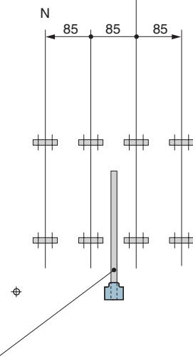
Horizontal terminals
